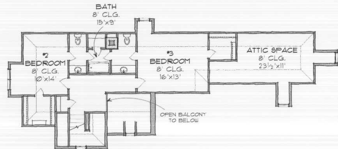
Upper Level Floor Plan
